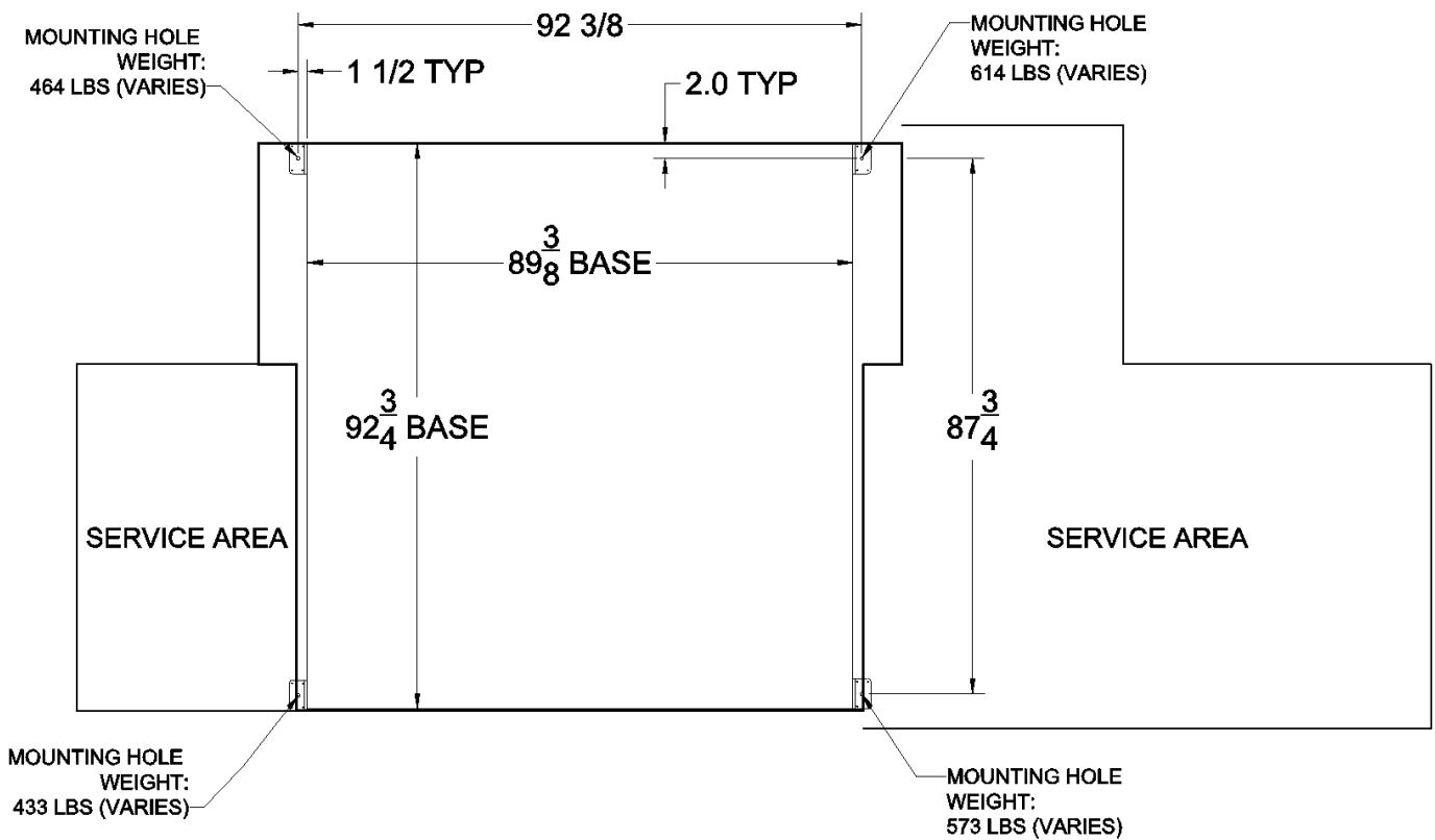
FIGURE 2-11 CORNER WEIGHTS
