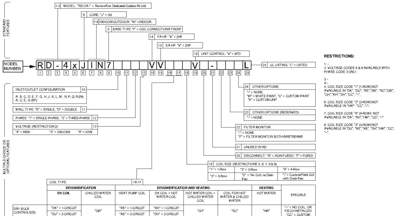
FIGURE 2-6: DIRECTORY TO RD4XIN MODEL NUMBERS
