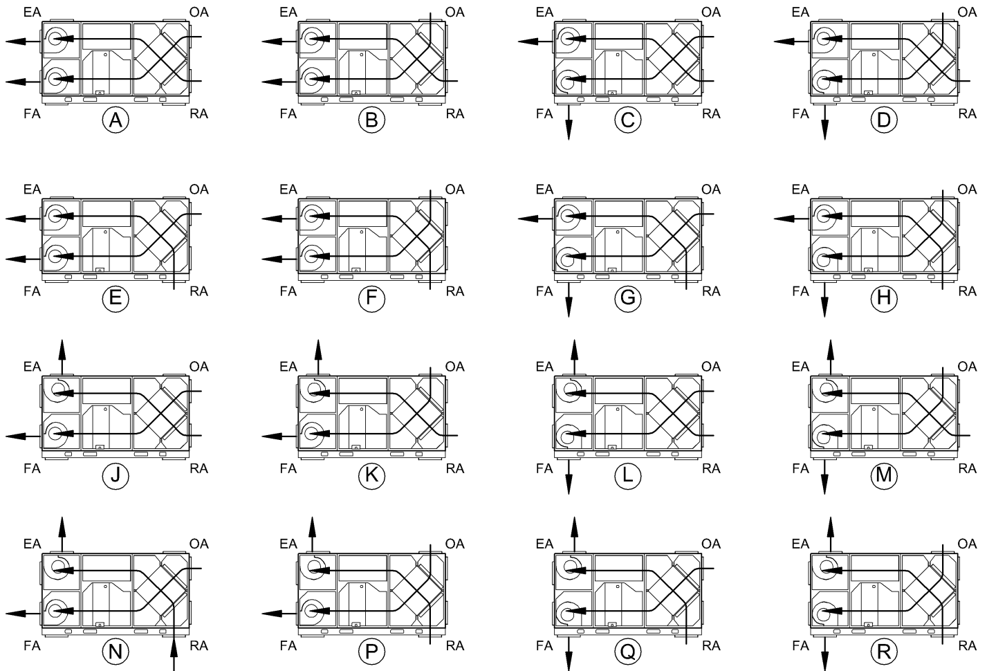
FIGURE 2-7 CHART OF ALL AVAILABLE INLET/OUTLET CONFIGURATIONS FOR RD4XIN
