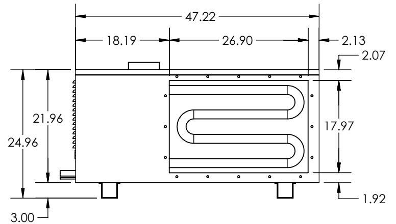
RIGHT VIEW
