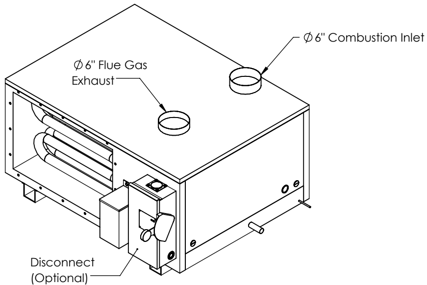
ISOMETRIC VIEW
