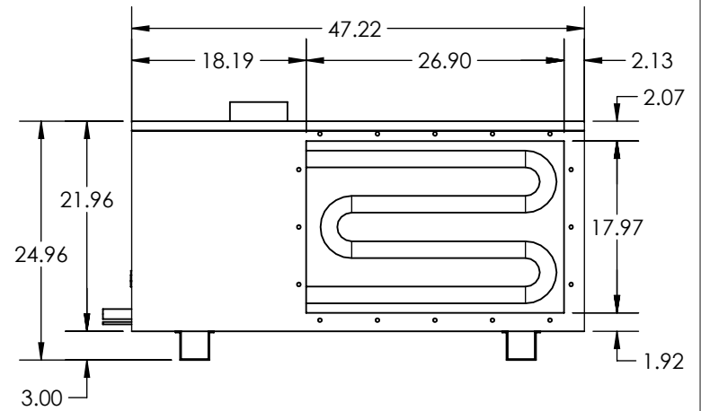
RIGHT VIEW
