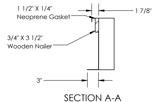
CURB CROSS-SECTION A-A (TYP.)
