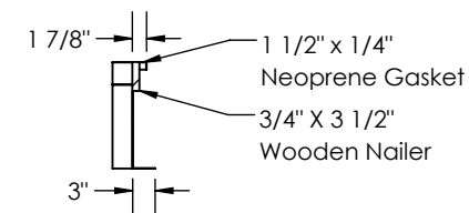
CURB CROSS-SECTION A-A (TYP.)
