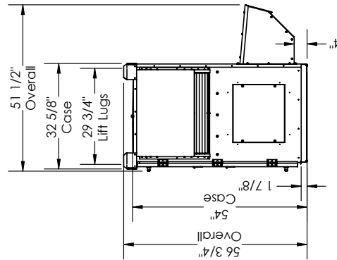
RIGHT VIEW
