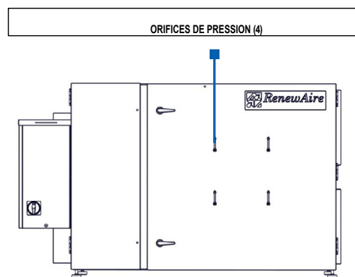
FIGURE 6.4.0 HE2XINV PRESSURE PORT LOCATIONS
