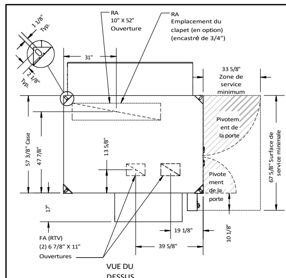
FIGURE 4.2.0 HE4XRT SERVICE CLEARANCE (TYP)
